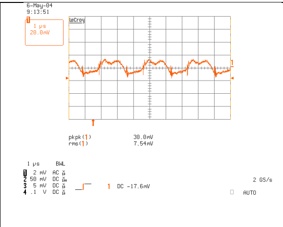
iEA48025A015V-000 Typical Output Ripple at nominal input voltage and full load at Ta=25 degrees
