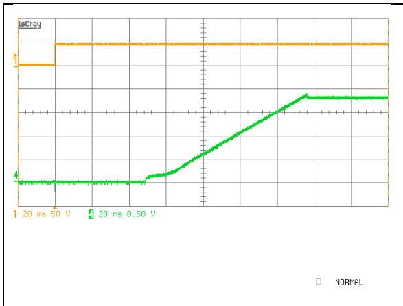
iEA48025A018V-000 Typical startup characteristic from input voltage application at full load. Ch1 - input voltage, Ch 4 – output voltage
