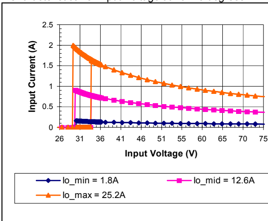
iEA48025A018V-000 Typical Input Current vs. Input Voltage Characteristics
