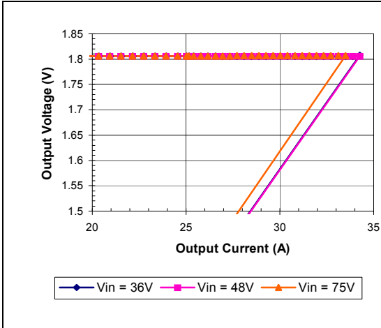
iEA48025A018V-000 Typical Output Current Limit Characteristics vs. Input Voltage at Ta=25 degrees.
