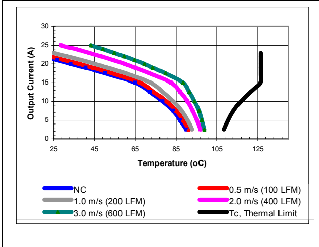
iEA48025A025V-000 maximum output current vs. ambient temperature at nominal input voltage for airflow rates natural convection (60lfm) to 600lfm with airflow from pin 3 to pin 1.
