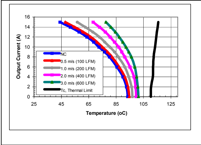
iEA48015A050V-000 maximum output current vs. ambient temperature at nominal input voltage for airflow rates natural convection (60lfm) to 600lfm with airflow from pin 3 to pin 1.
