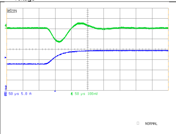
iEA48025A018V-000 Typical transient response. Output voltage response to load step from 50% to 75% of full load with output current slew rate of 0.1A/ \mu S.
